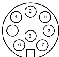
VIEW INTO RADIO JACK (VIEW INTO BACK OF PLUG)
